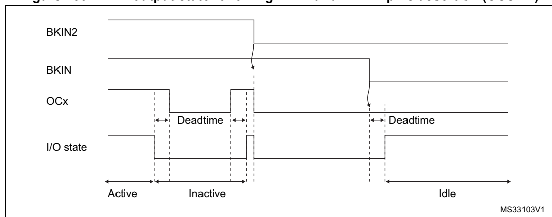
Figure 183. PWM output state following BKIN and BKIN2 pins assertion ( OSSI=1 )
